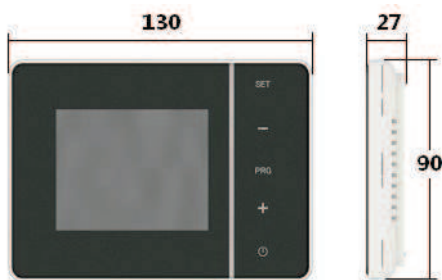
Fig.2: Dimensional Diagram – Length, Width, Thickness, Installing Size
