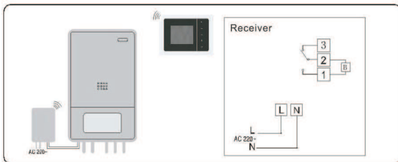
Fig.4: Control of Wall-mounted Boiler for HY01RFB mode
