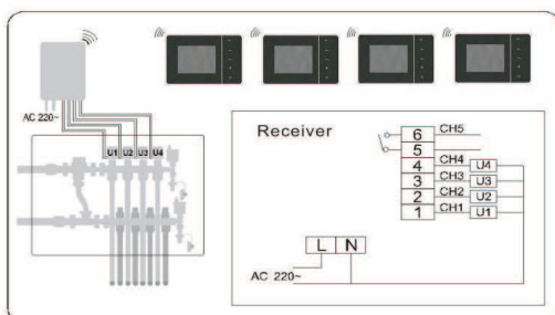
Fig.5: Control of Under Floor Heating with Wireless 4-channel for MRF mod
